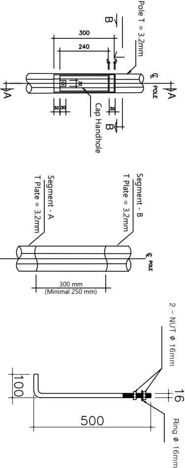
Det.2. Handhole SCALE 1 : 25
